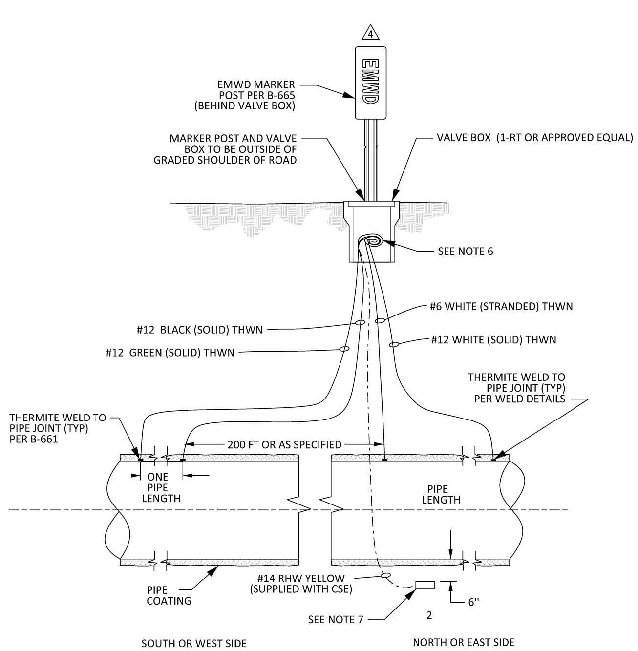
LINE CURRENT TEST STATION NOT TO SCALE
