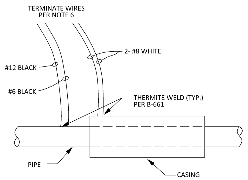
PIPE W/CASING TEST STATION NOT TO SCALE
