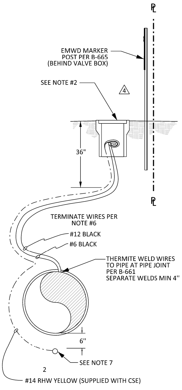
BASIC TEST STATION NOT TO SCALE
