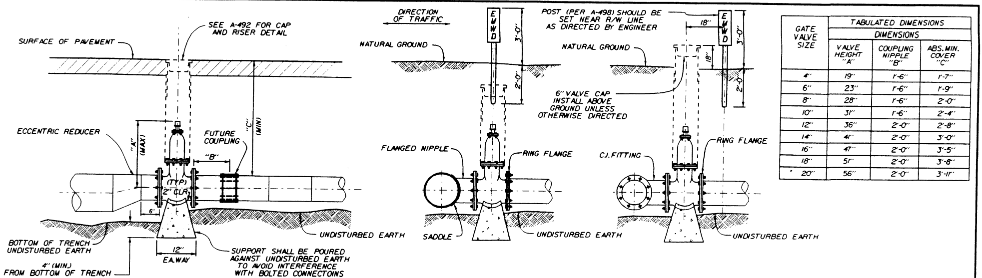
IN-LINE VALVE INSTALLATION SADDLE OUTLET INSTALLATION C.J. FITTING INSTALLATION
