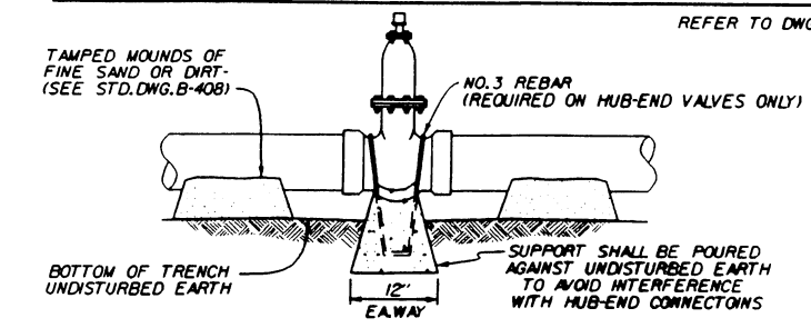
AC-P.V.C. & D.I.P. PIPELINE INSTALLATION FOR 4" DIAMETER AND LARGER
