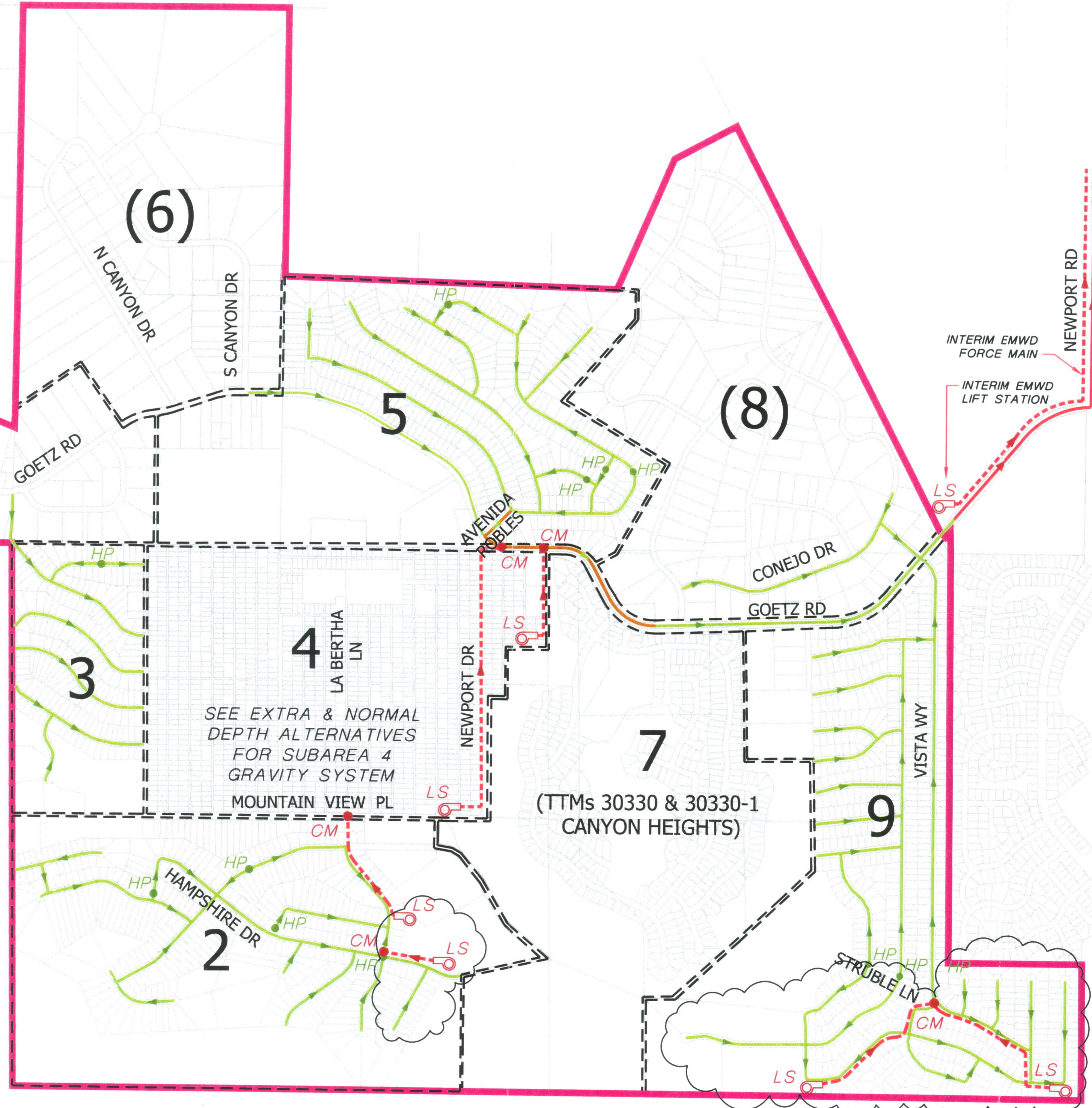
QUAIL VALLEY EMWD GRAVITY SYSTEM OVERALL STUDY AREA BY: KJO - DATE 10/05 FIG. 5
