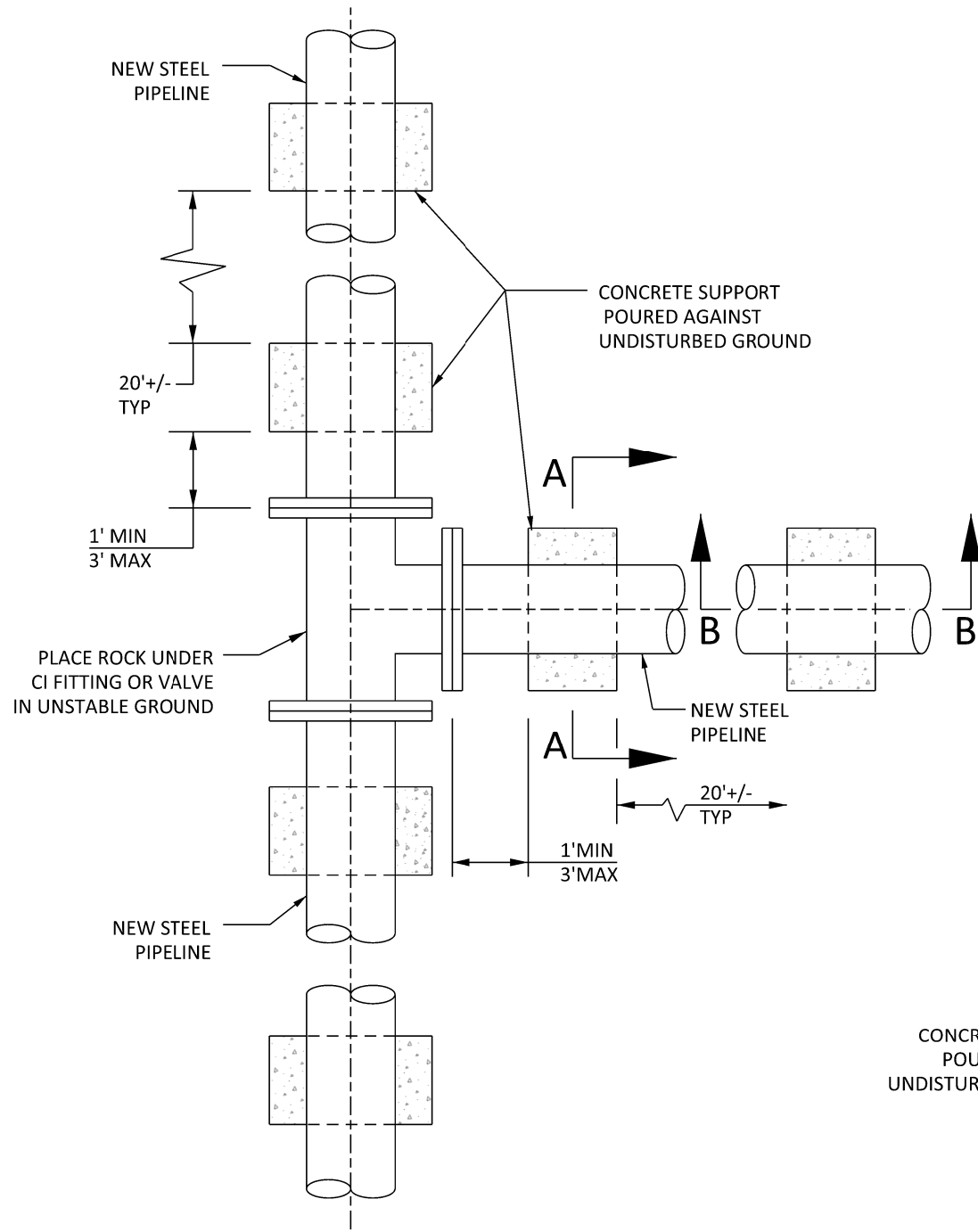
NEW STEEL PIPELINE INSTALLATION
